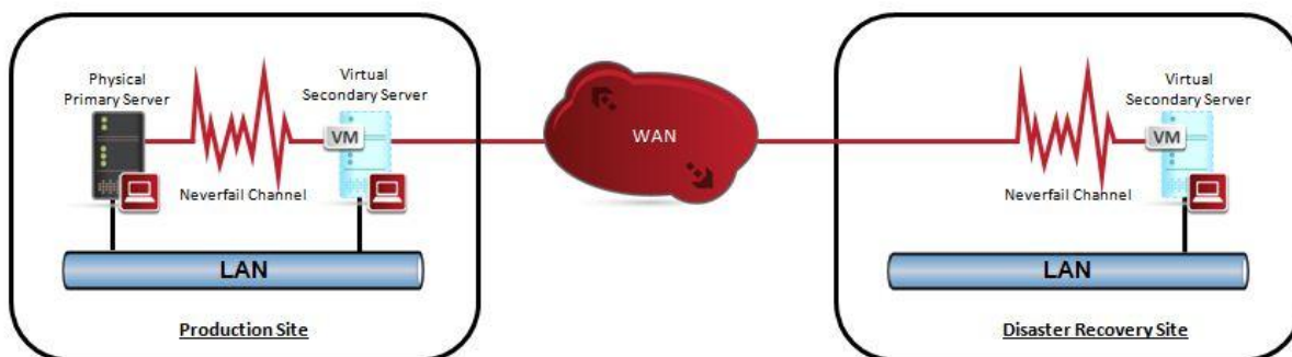
Figure 8 – Protecting mixed physical, virtual servers with local & remote site availability (P2V2V)
