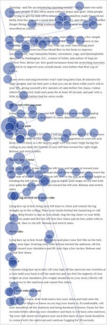
Gaze plot
